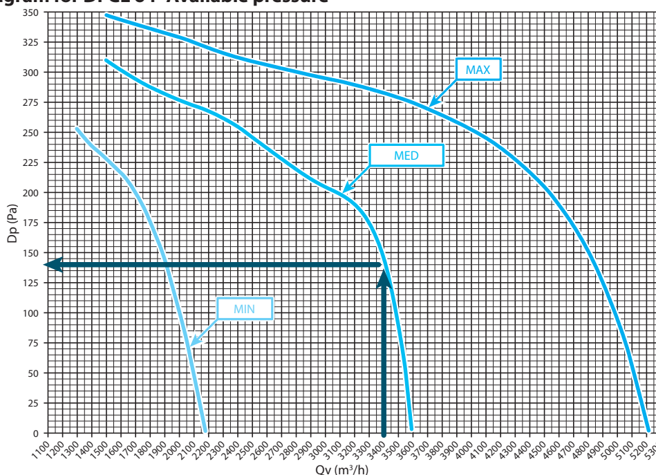
Diagram for DFCL 64 "Available pressure"
