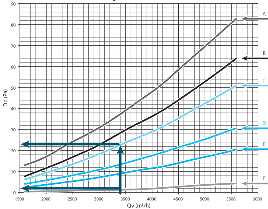
Diagram for DFCL 64 "Pressure drop"
