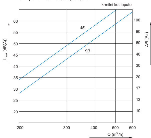
OD-4/S velikost 400,500,600,625
