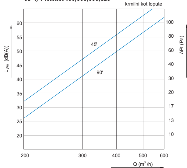
OD-4/V velikost 400,500,600,625
